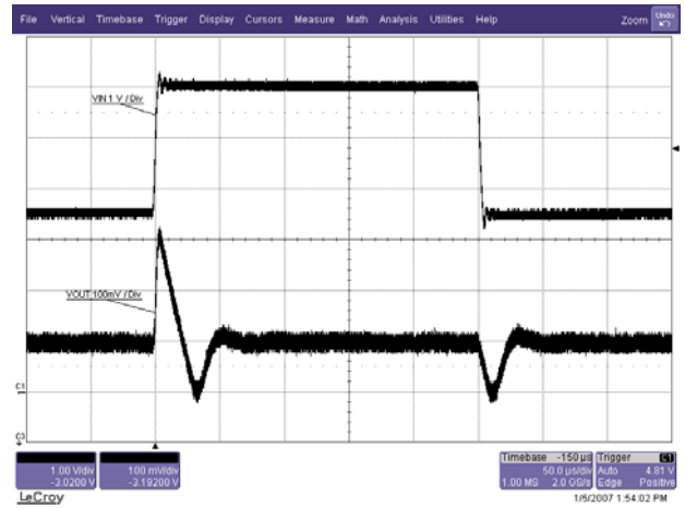
Figure 9. Line Transient Response
